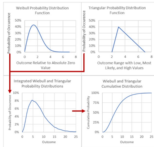
Figure 3. Combining Distributions Example
