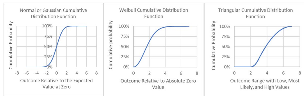
Figure 2. Cumulative Distribution Function (CDF) Examples
