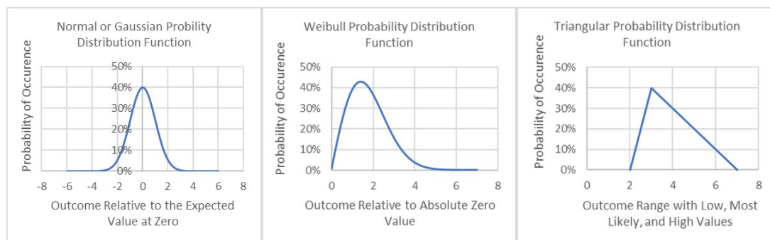
Figure 1. Probability Distribution Function (PDF) Examples
